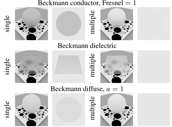
Figure 16: White furnace test for different microfacet materials.
